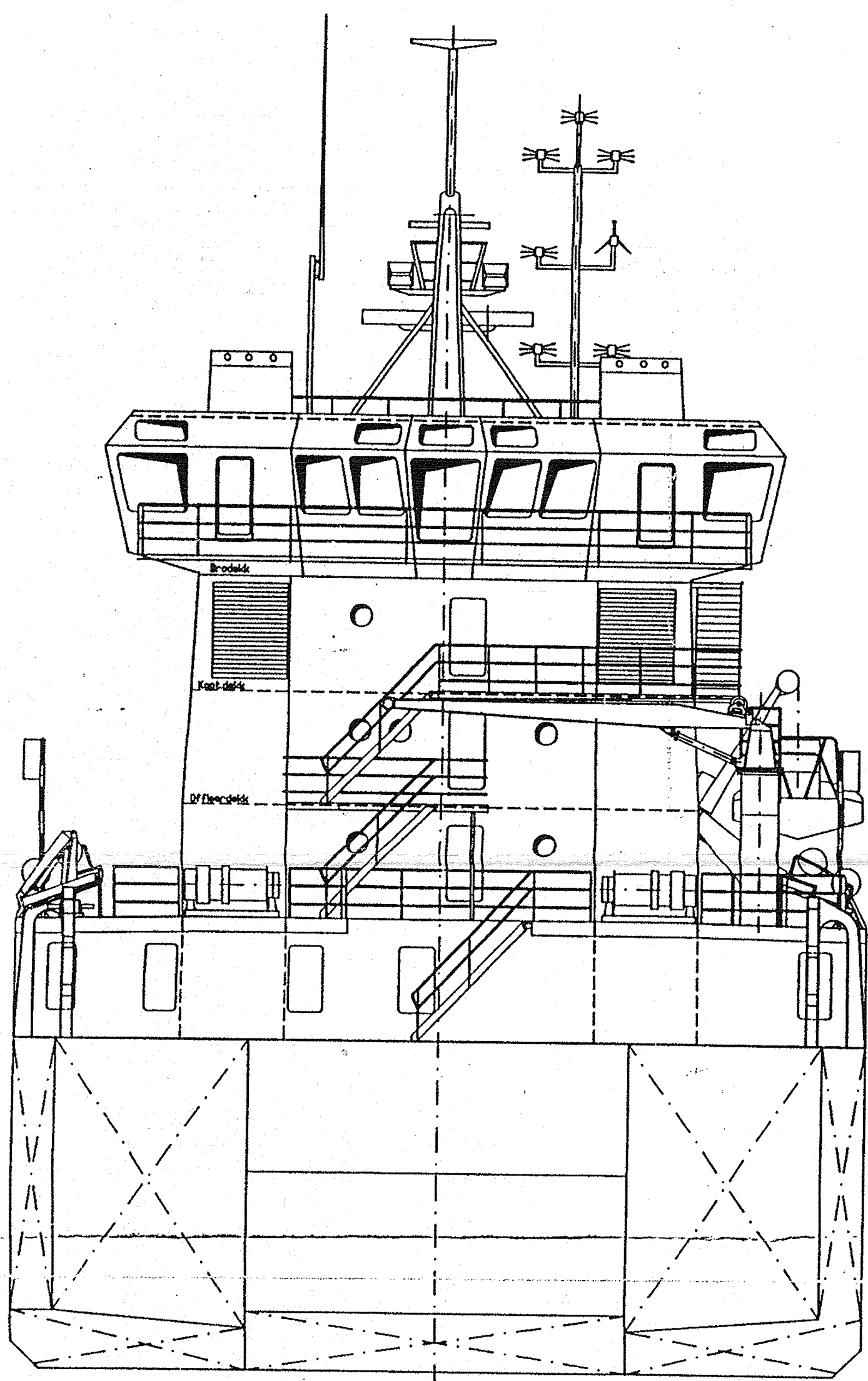
STERN ELEVATION
