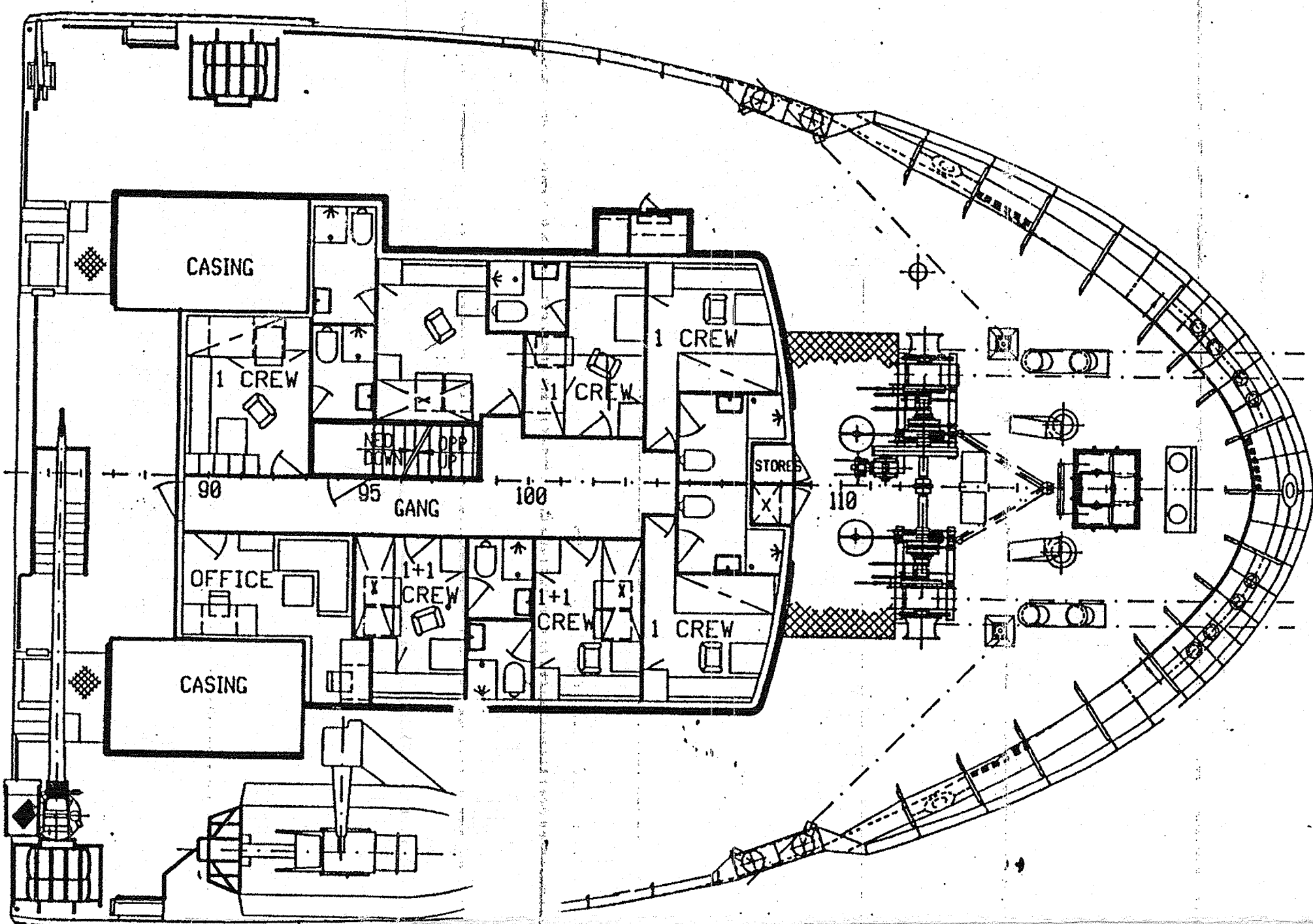
FORECASTLE DECK
