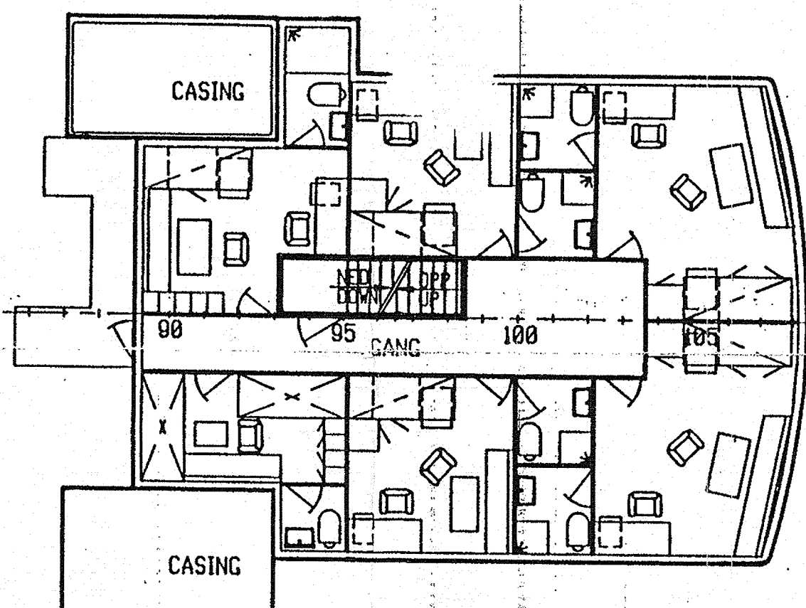
OFFICER'S DECK
