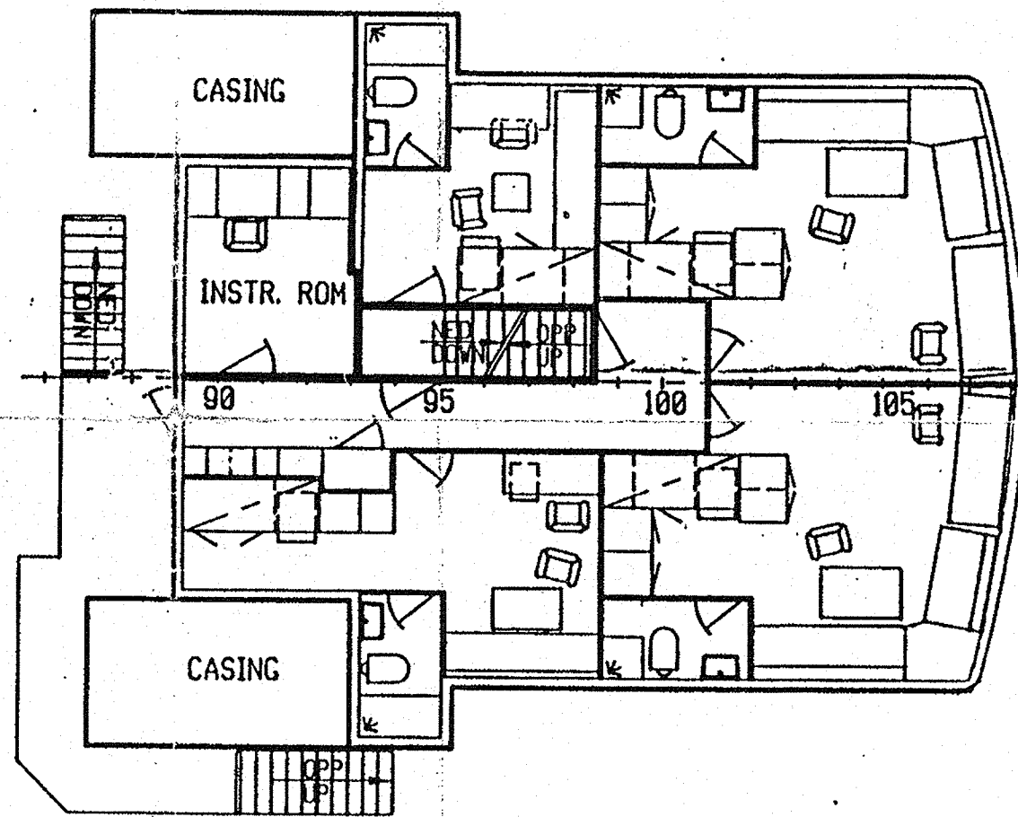
CAPTAIN'S DECK
