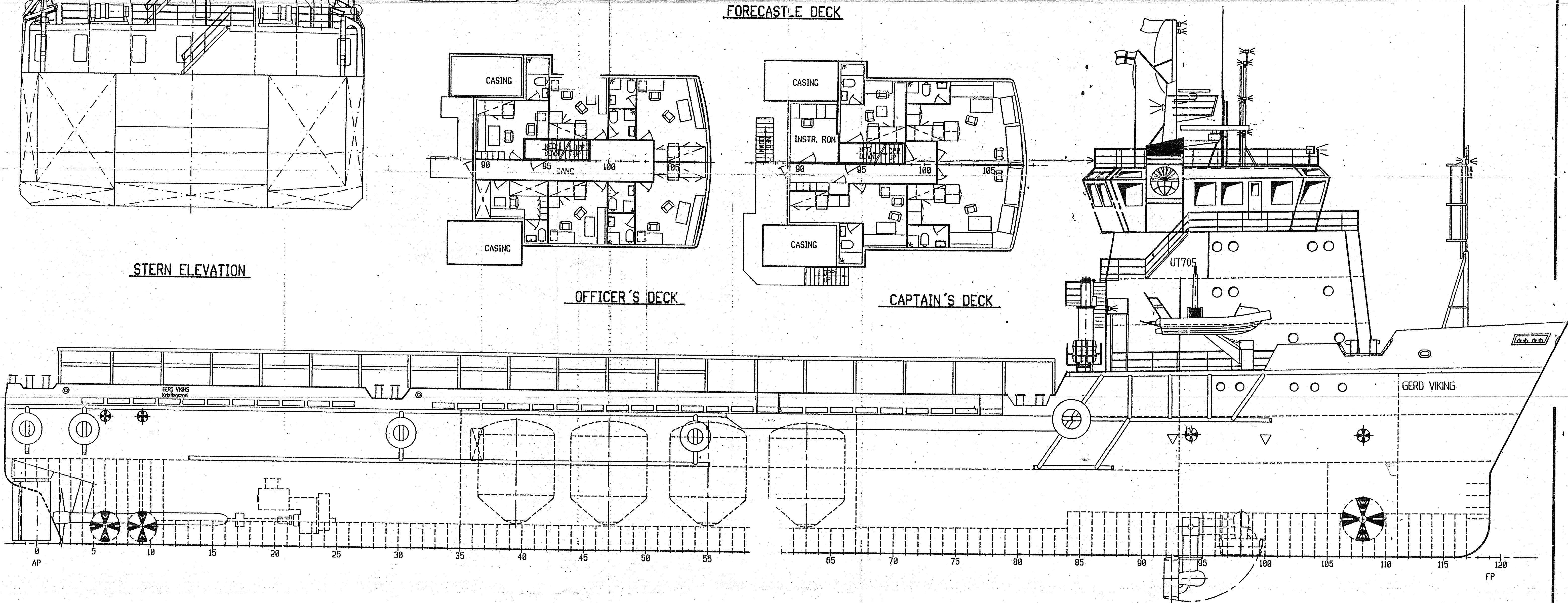
FORECASTLE DECK
