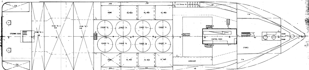
MAIN DECK
