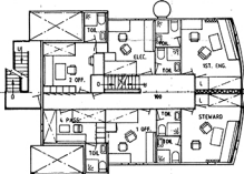
OFFICERS DECK
