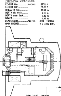
BRIDGE DECK
