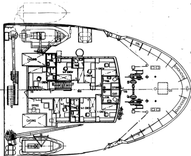
FORECASTLE DECK
