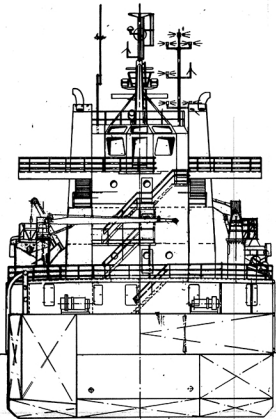
STERN ELEVATION
