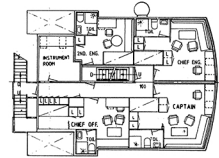
CAPTAIN DECK
